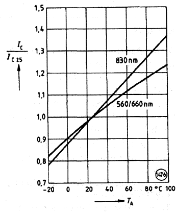
Photocurrent I_C / I_{C25} = f(T_A), V_{CE} = 5 \text{ V}, \lambda = \text{parameter}
