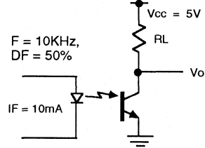
Figure 2. Saturated switching timing
