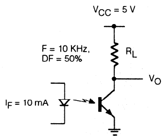
Figure 10. Switching schematic
