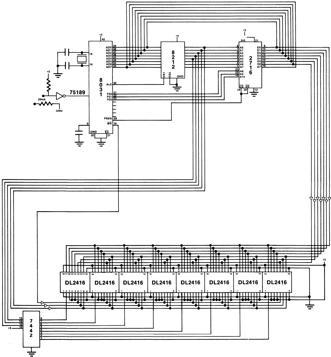
FIGURE 3 — SYSTEM SCHEMATIC
