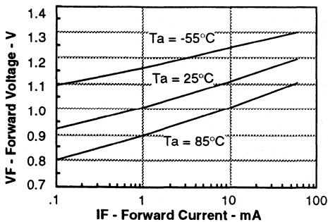
Figure 5. Forward voltage versus forward current
