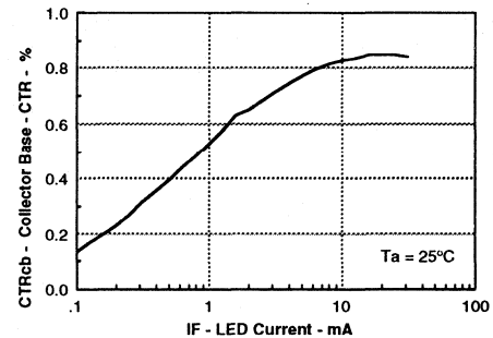
Figure 6. Collector base current transfer ratio versus LED current
