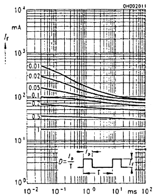
8B Permissible pulse handling capability I_F=f(t_p) , T_A=25^\circ\text{C} ; Duty cycle D=\text{parameter}
