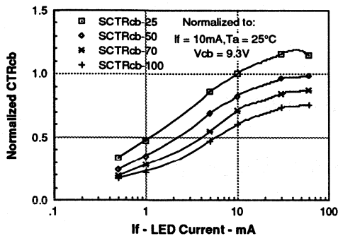
Figure 6. Normalized CTR CB versus LED Current
