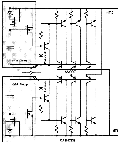
Figure 9. Schematic
