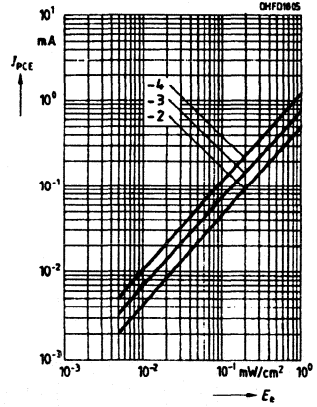
Photocurrent I_{PCE}=f(E_E), V_{CE}=5\text{ V}
