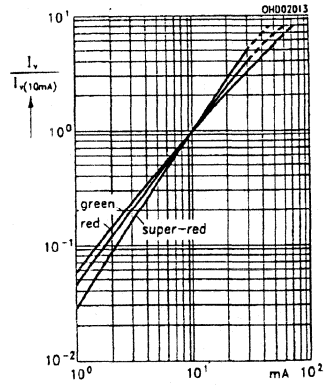
6A Relative luminous intensity I_v/I_{v(10\text{mA})}=f(I_f), T_A=25^\circ\text{C}
