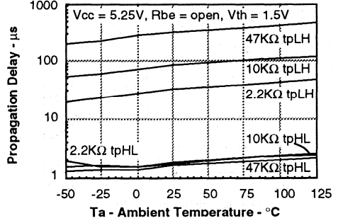
Figure 16. Saturated Switching
