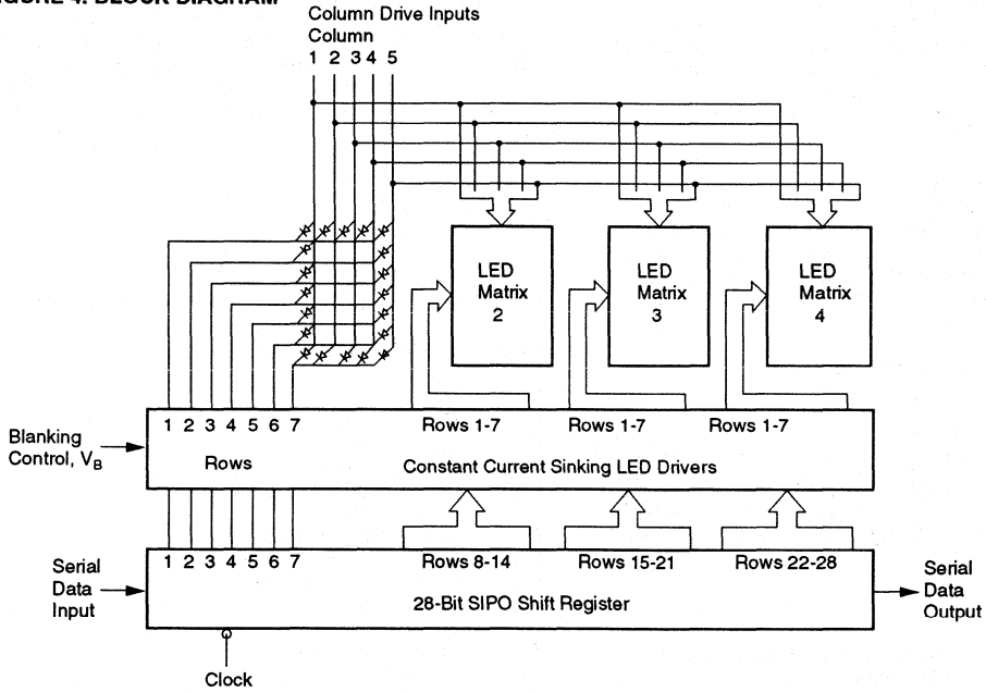
FIGURE 4. BLOCK DIAGRAM
