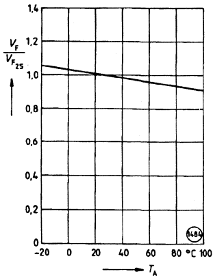
Forward voltage-SFH452V
