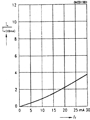
6F Relative luminous intensity I_v/I_{v(10\text{mA})}=f(I_f), T_A=25^\circ\text{C}
