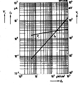
BPX 48F Photocurrent I_p=f(E_v) , V_R=5 V Open circuit voltage V_O=f(E_v)
