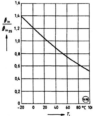
Temperature behavior—SFH750V
