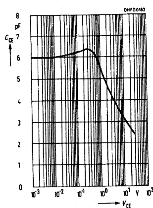
Collector emitter capacitance C_{CE}=f(V_{CE}) , f=1\text{ MHz} , E=0
