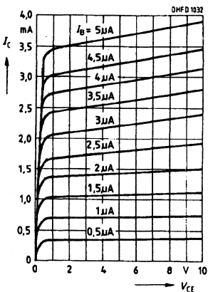
Output characteristics I_C=f(V_{CE}), I_B=\text{Parameter}
