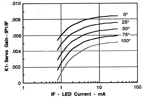
Figure 3. Servo Gain vs. LED Current
