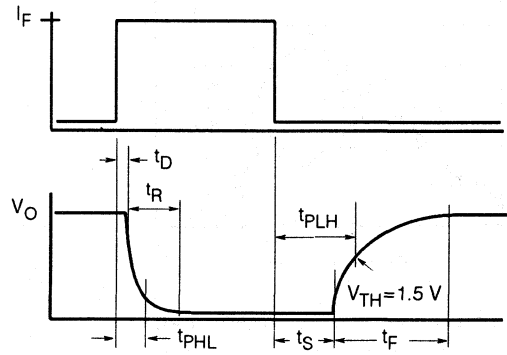
Figure 16. Switching timing
