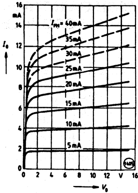
Figure 5. Forward current of emitting diode versus current forward voltage ( T_A=25^\circ\text{C} )
