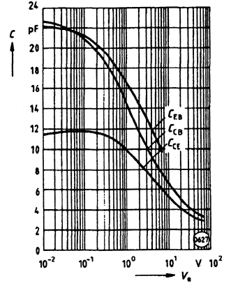
Figure 18. Transistor capacitance C=f(V_O) ( T_A=25^\circ\text{C} , f=1\text{ MHz} )
