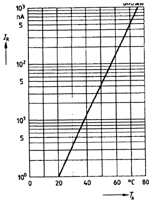
Dark current versus ambient temperature I_R=f(T_A), V_R=5 V
