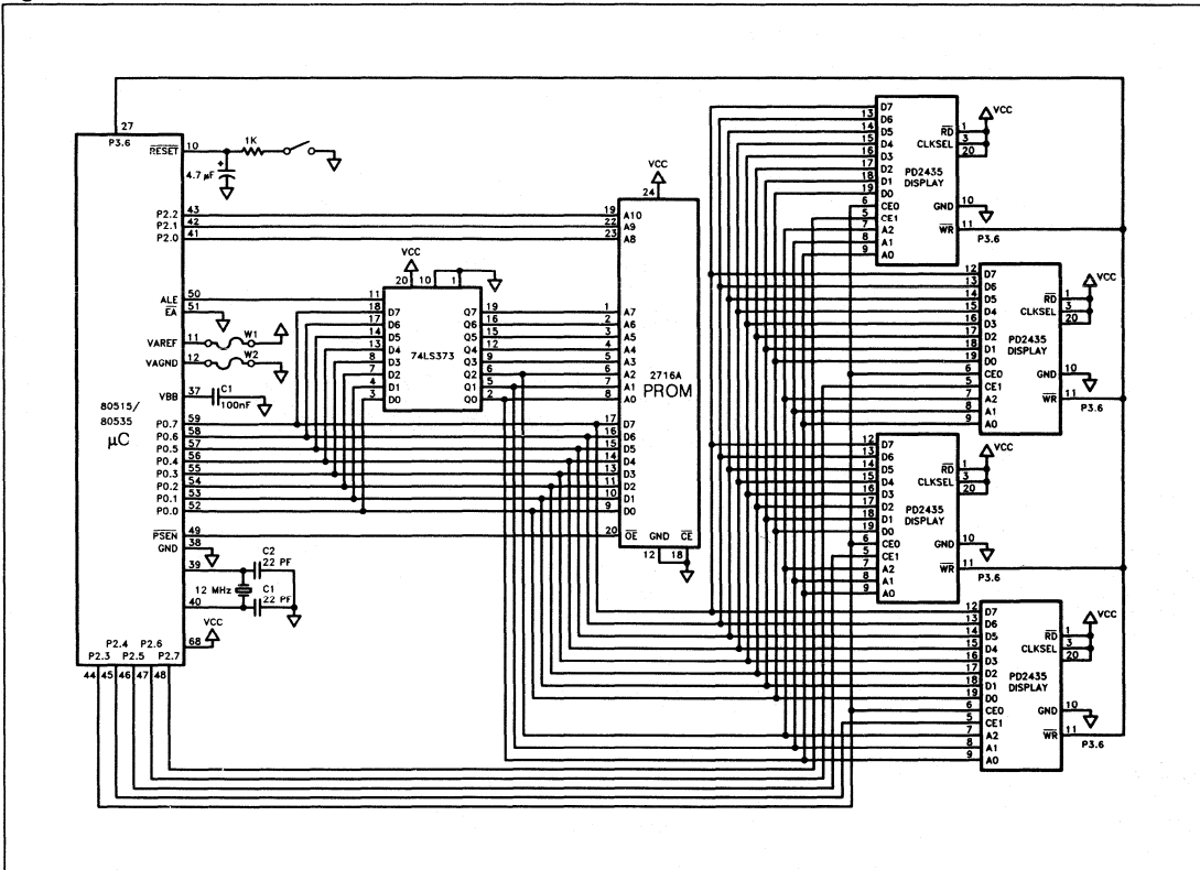
Figure 4. Interface Circuit
