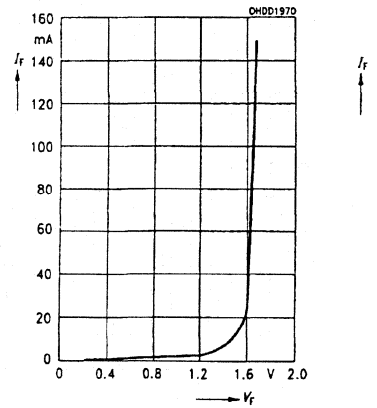
3C Forward current I_F=f(V_F) , T_A=25^\circ\text{C}
