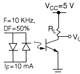
Figure 15. Switching schematic
