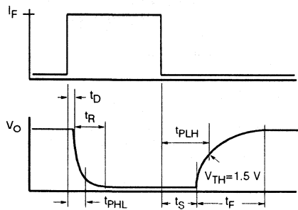
Figure 9. Switching timing
