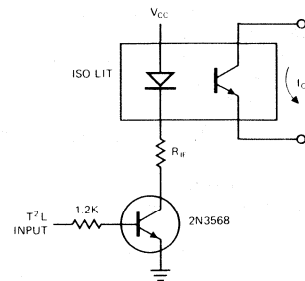
Figure 1A. NPN Driver
