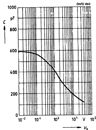
Capacitance C=f(V_R), f=1 MHz
