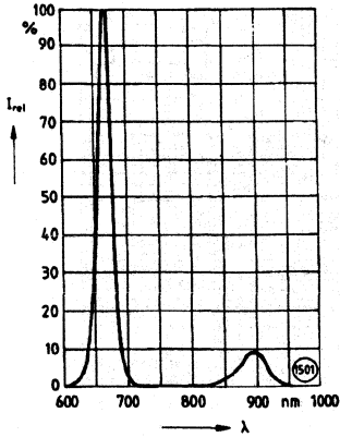
Relative optical output power
