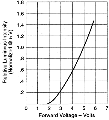
Relative luminous intensity versus forward voltage
