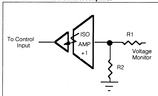
FIGURE 16. Isolated Control Amplifier
