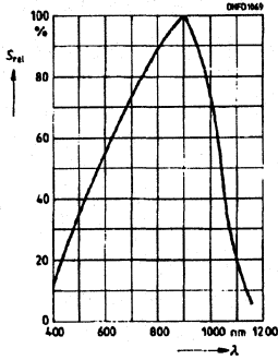
BPX 48 Relative spectral sensitivity S_{REL}=f(\lambda)
