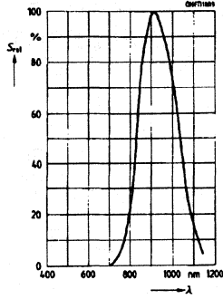
BPX 48F Relative spectral sensitivity S_{REL}=f(\lambda)
