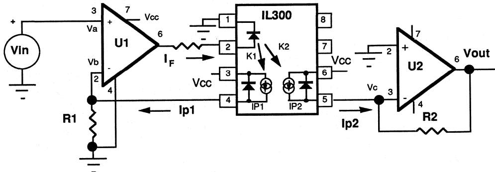
Figure 7. Composite Amplifier
