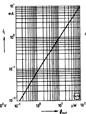
Photocurrent I_C = f(\Phi_{OUT}), V_{CE} = 5 \text{ V}, \lambda = 560 \text{ to } 950 \text{ nm}
