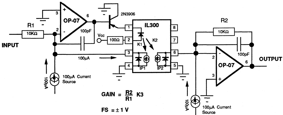
Figure 18. Prebiased Photovoltaic Isolation Amplifier
