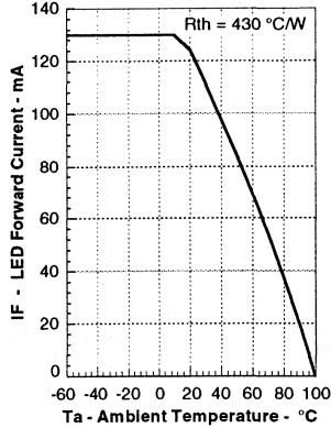
Figure 2. Maximum LED current versus ambient temperature
