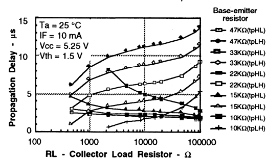
Figure 30. Propagation delay versus collector load and base-emitter resistance for I_f=10 mA
