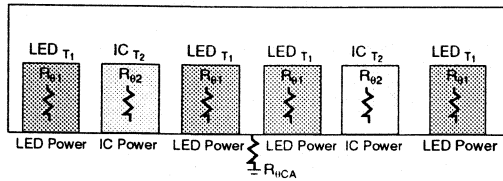
FIGURE 5. THERMAL MODEL
