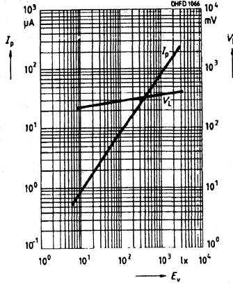
Photocurrent I_P = f(E_V)
