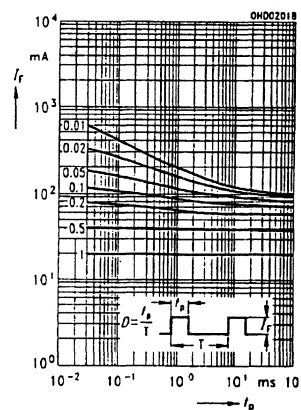
8G Permissible pulse handling capability I_F=f(t_p) , T_A=25^\circ\text{C} ; Duty cycle D=\text{parameter}
