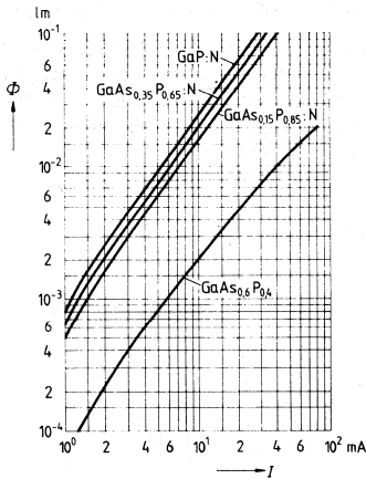
Fig. 2.5 Light current – diode current characteristic
