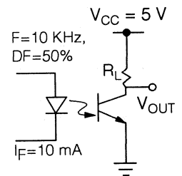
Figure 9. Switching schematic
