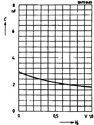
Capacitance C=f(V_R), f=1 \text{ MHz}, E=0
