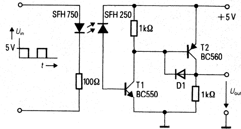
Fig. 9 Amplifier with common-emitter circuit suitable for analog signals up to 50 kHz
