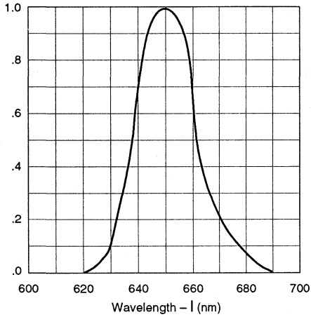
Spectral distribution
