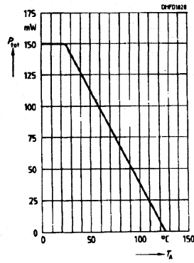
Power dissipation P_{TOT}=f(T_A) KOM 2033AF/2100AF
