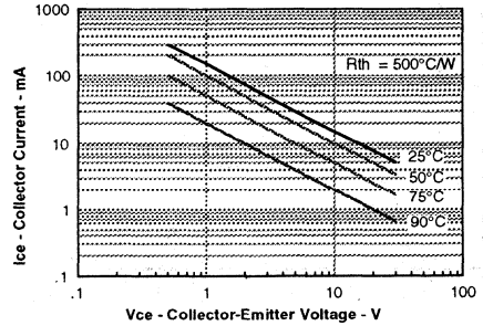
Figure 10. Maximum collector current versus collector voltage
