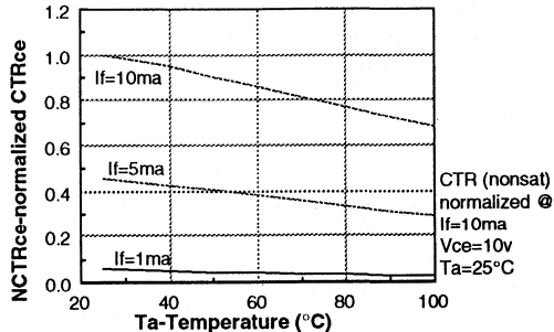
Figure 6. Collector current versus temperature
