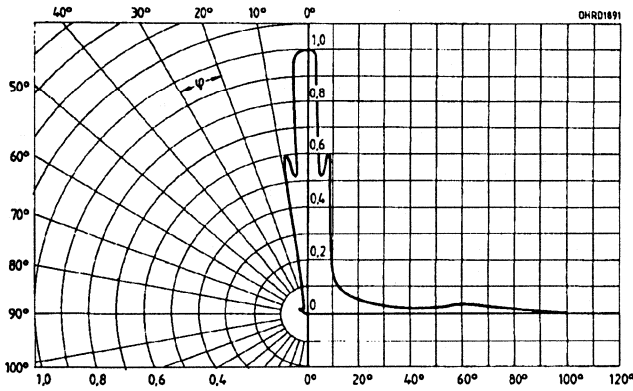
SFH 484—Radiation characteristic I_{REL} = f(\varphi)
