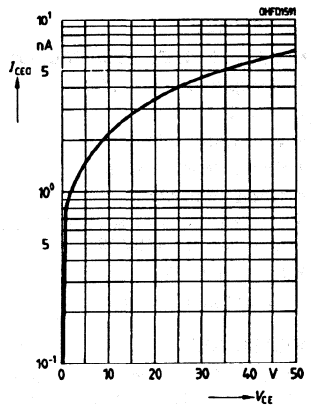
Dark current I_{CEO}=f(V_{CE}) , E=0
