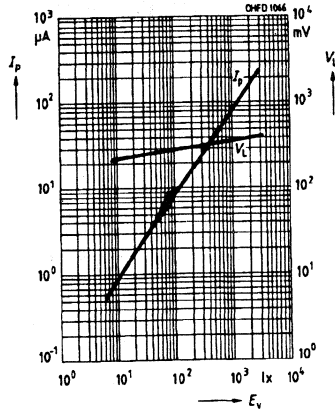
Photocurrent, I_p=f(E_v), V_a=5\text{ V} Open circuit voltage, V_L=f(E_v)
