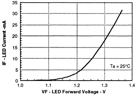
Figure 1. LED forward current versus forward voltage
