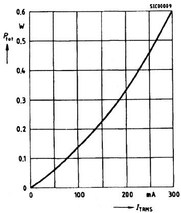
Figure 12. Power dissipation 40 to 60 Hz line operation, P_{TOT} = f(I_{TRMS})
