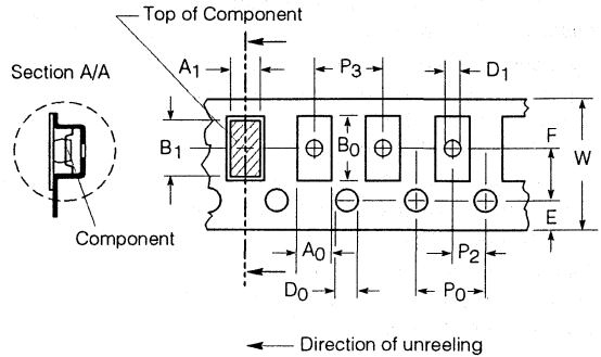
Blister Tape
