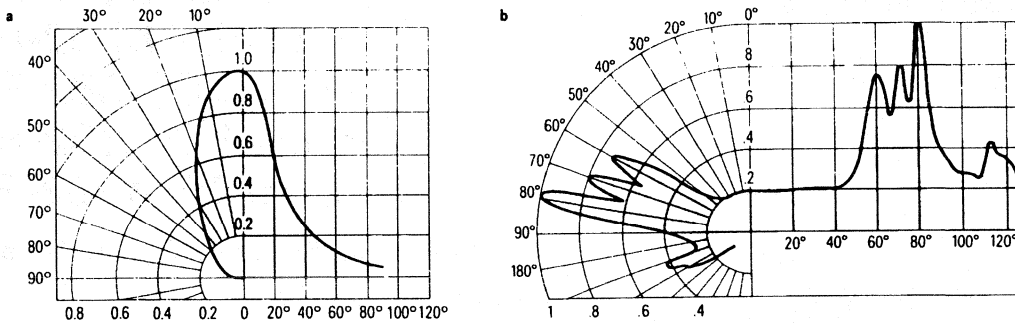
FIGURE 1. ARGUS LEDs emit their light over an enlarged solid angle. Both graphs show polar coordinates on the left and rectangular coordinates on the right. a) Standard LED-viewing angle b) ARGUS LED-radiation characteristic. Relative spatial emission vs. half angle.
