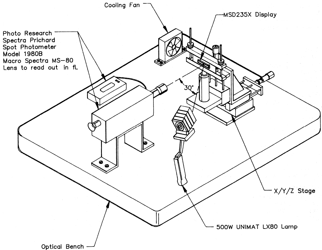
Figure 1. Sunlight Readability Contrast Measurement Setup
