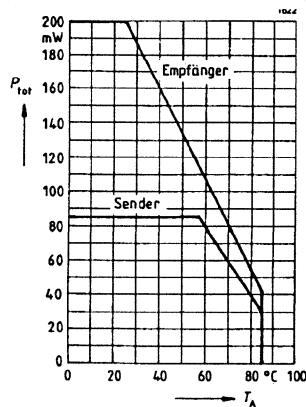
Permissible power dissipation P_{TOT} = f(T_A)
