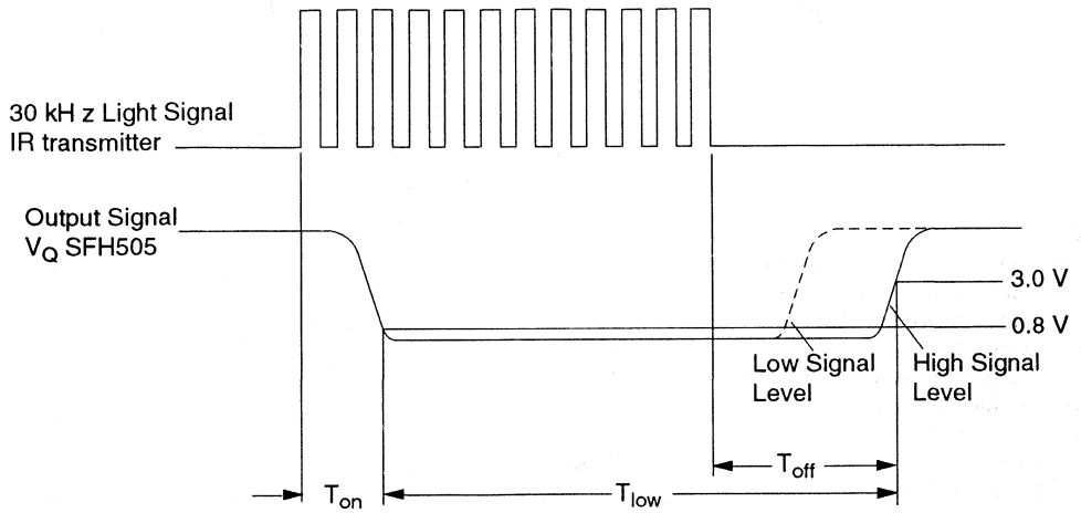
Figure 2. Timing Diagram
