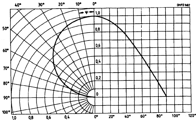
Directional characteristics S_{rel}=f(\beta)
