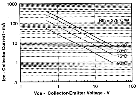
Figure 7. Collector current versus collector-emitter voltage
