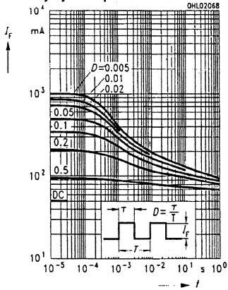
5G Permissible pulse handling capability I_F=f(t_p) , T_A=25^\circ\text{C} Duty cycle d -parameter
