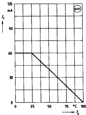
Figure 7. Permissible diode forward current versus ambient temperature
