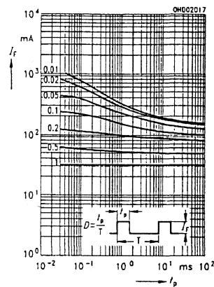
8F Permissible pulse handling capability I_F=f(t_p) , T_A=25^\circ\text{C} ; Duty cycle D=\text{parameter}
