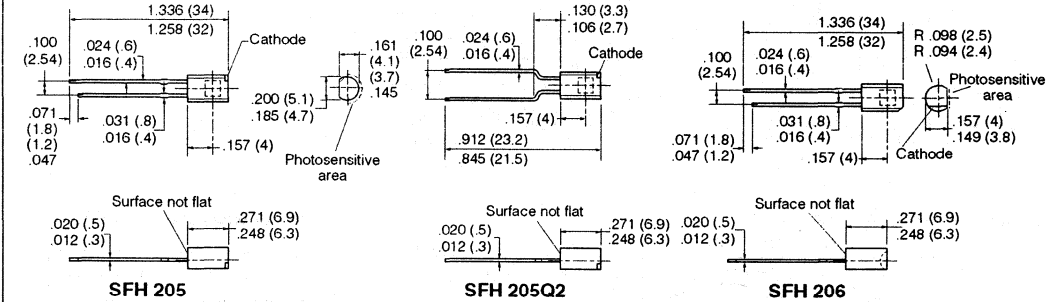
Package Dimensions in Inches (mm)
