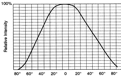
Radiation characteristics
