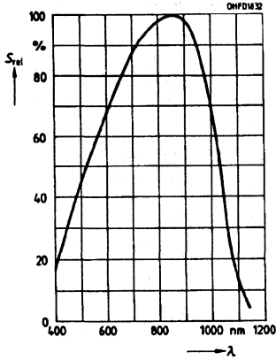
Relative spectral sensitivity S_{rel}=f(\lambda) KOM 2033B/2100B
