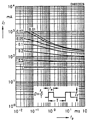
8E Permissible pulse handling capability I_F=f(t_p) , T_A=25^\circ\text{C} ; Duty cycle D=\text{parameter}
