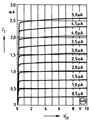
Output characteristics I_C = f(V_{CE}), I_B = \text{parameter}
