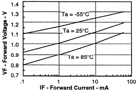
Figure 4. Forward voltage versus forward current
