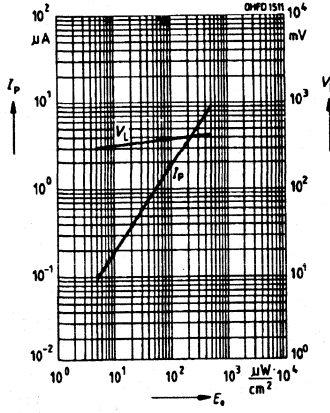
Photocurrent I_P=f(E_E) , V_R=5\text{ V} , Open-circuit voltage V_L=f(E_E) SFH229F
