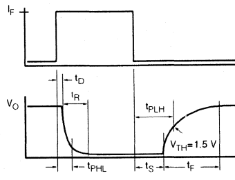
Figure 8. Switching waveform
