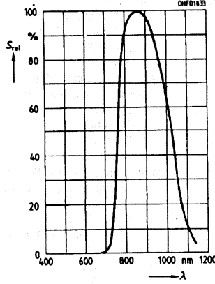
Relative spectral sensitivity S_{rel}=f(\lambda) KOM 2033BF/2100BF
