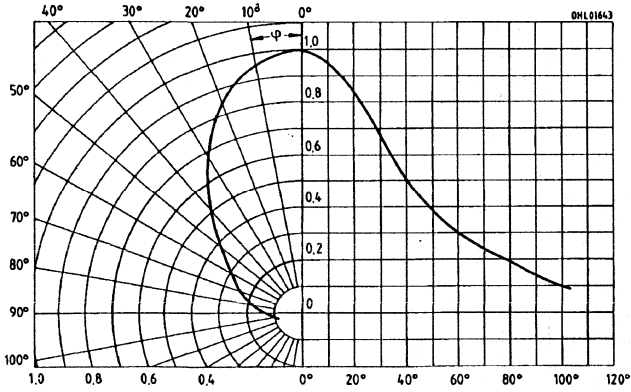
Radiation characteristics I_{rel}=f(\rho)
