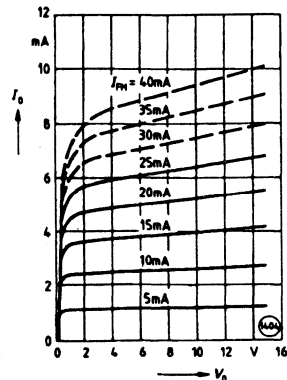
Figure 1. Output characteristics—SFH6135
