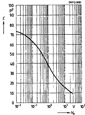
Capacitance C = f(V_R)
