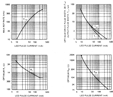
Figure 3. Parameters vs LED Pulse Current
