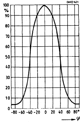
Radiation characteristics S_{REL}=f(\varphi)
