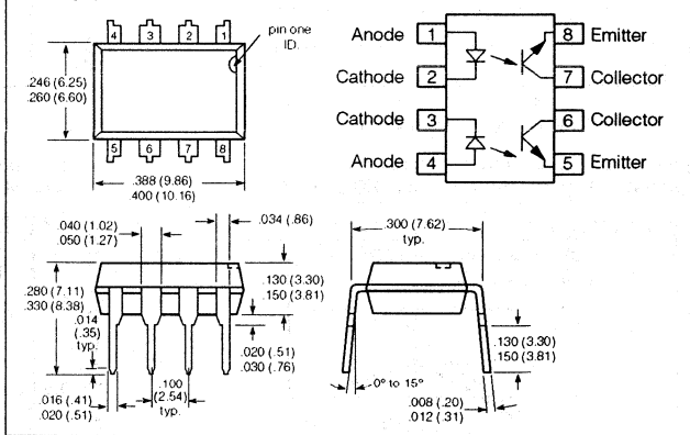
Package Dimensions in Inches (mm)
