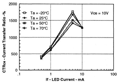
Figure 6. CTR versus LED current
