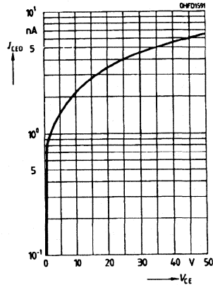
Dark current I_{CEO}=f(V_{CE}), E=0
