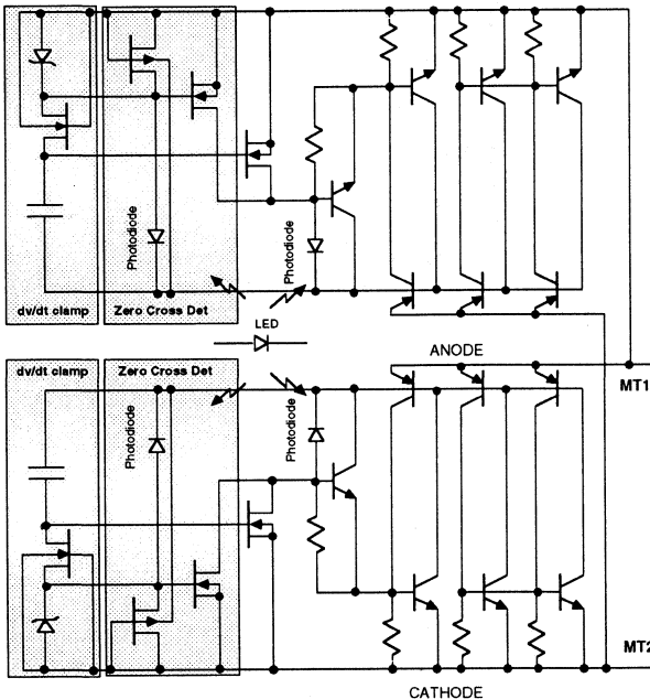
Figure 9. Schematic
