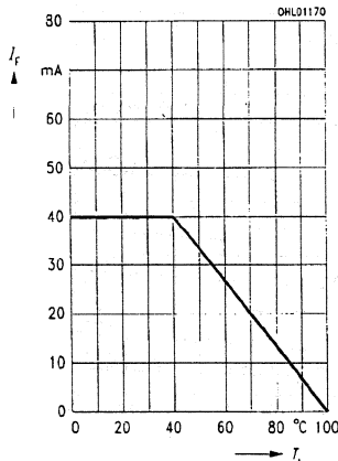
6A Max. permissible forward current I_F=f(T_A)
