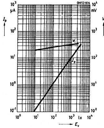
Photocurrent I_P=f(E_V) , V_R=5V Open circuit voltage V_O=f(E_V)
