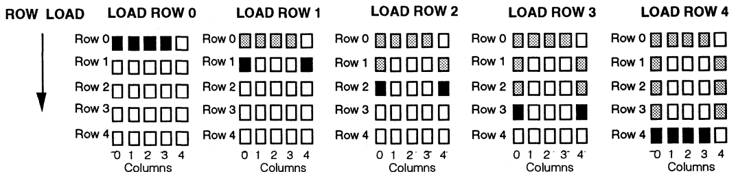
FIGURE 9. ROW STROBING
