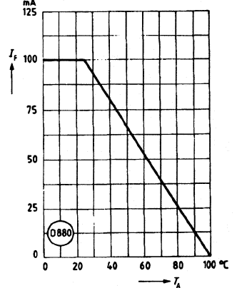
Maximum permissible forward current—SFH452V I_F=f(T_A)
