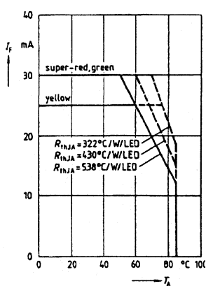
9L Maximum permissible forward current I_F=f(T_A)
