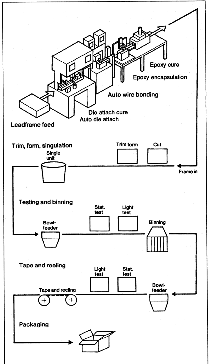
Figure 19. Manufacturing process flow.
