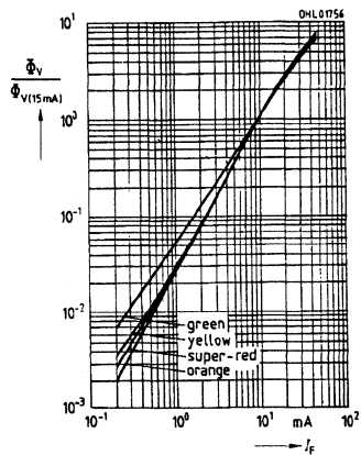
4H Rel. luminous flux \Phi_V/\Phi_V(15\text{ mA}) = f(I_F)
