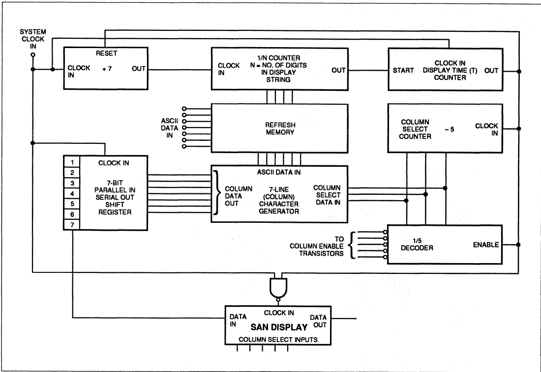
Figure 2. Block Diagram
