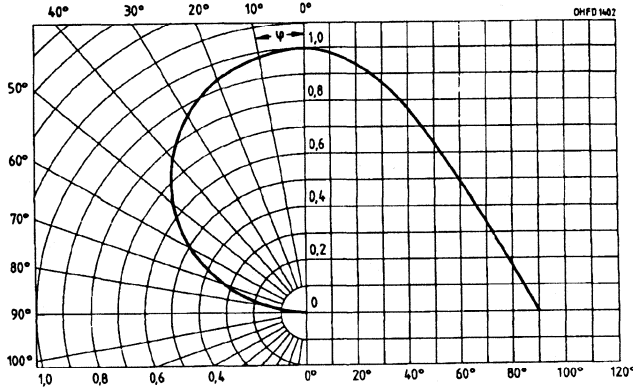
Directional characteristics S_{rel}=f(\theta)
