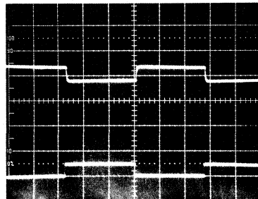
U_C = 1 \text{ V/Div} I_F = 10 \text{ mA/Div} t = 10 \text{ μs/Div}
