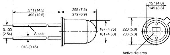
Package Dimensions in Inches (mm)
