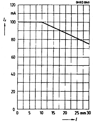
Forward current vs. lead length, package bottom and PC-board I_F = f(l) , T_A = 25^\circ\text{C}
