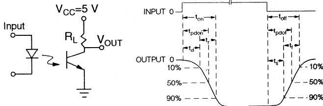
Figure 8. Switching time test schematic and waveform
