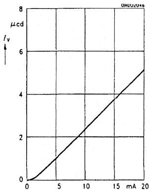
7A Luminous intensity I_V=f(I_F) , T_A=25^\circ\text{C}
