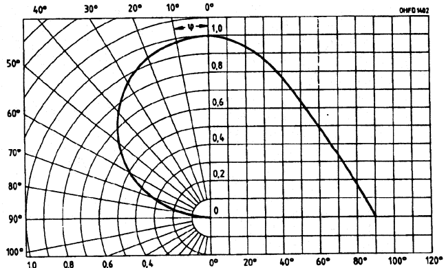
Directional characteristics S_{REL}=f(\varphi)
