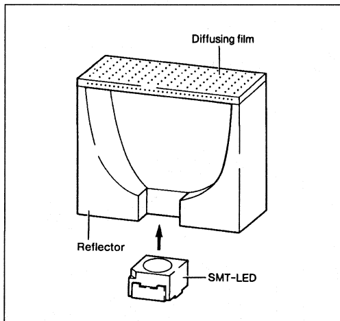
Figure 9. SMT-TOPLED™ illuminating a reflecting cavity.
