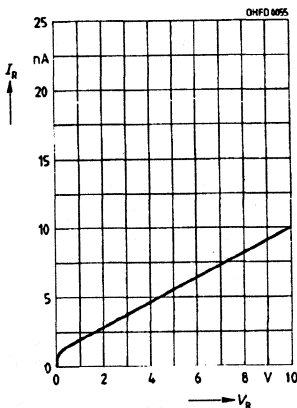
Dark current I_R=f(V_R) , f=1 MHz, E=0
