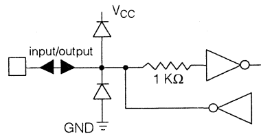
FIGURE 4. CLOCK I/O
