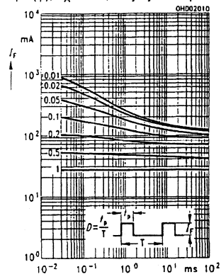
8A Permissible pulse handling capability I_F=f(t_p) , T_A=25^\circ\text{C} ; Duty cycle D=\text{parameter}
