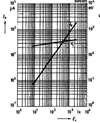
Photocurrent I_P=f(E_V) , V_R=5\text{ V} Open circuit voltage V_0=f(E_V)
