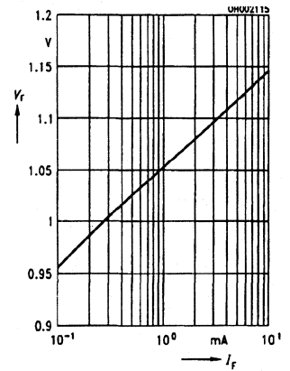
Figure 3. Diode forward voltage T_A=25^\circ\text{C} , V_F=f(I_F)
