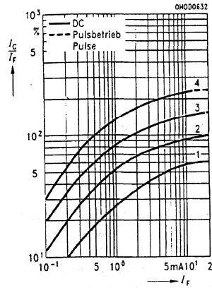
Figure 2. Current transfer ratio versus diode current ( T_A=0^\circ\text{C} , V_{CE}=5\text{ V} ) I_C/I_F=f(I_F)
