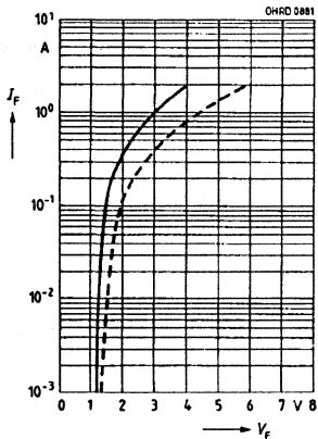
Forward current I_F = f(V_F) Single pulse, \tau = 20 \mu\text{s}
