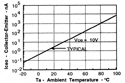
Figure 15. Collector-emitter leakage versus temperature
