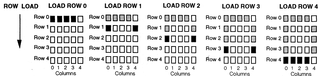
FIGURE 9. ROW STROBING
