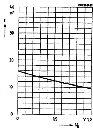
Capacitance C=f(V_R), f=1 \text{ MH}, E=0
