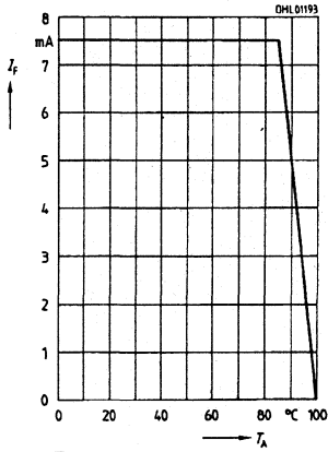
6F Max. Permissible forward current I_F=f(T_A)
