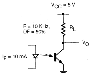
Figure 15. Switching Schematic
