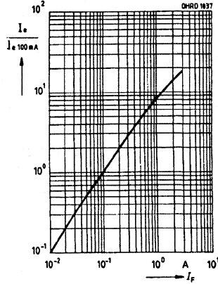
Radiant Intensity I_E / I_{E50mA} = f(I_F) Single pulse, \tau = 20 \mu s
