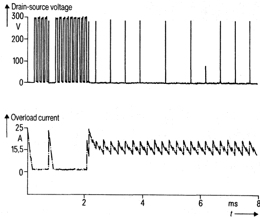
Fig. 6 Current and voltage waveforms in the FREDFET with overload
