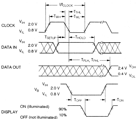
FIGURE 1. TIMING CHARACTERISTICS
