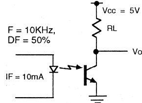
Figure 4. Saturated switching timing
