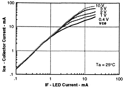
Figure 11. Transfer curve
