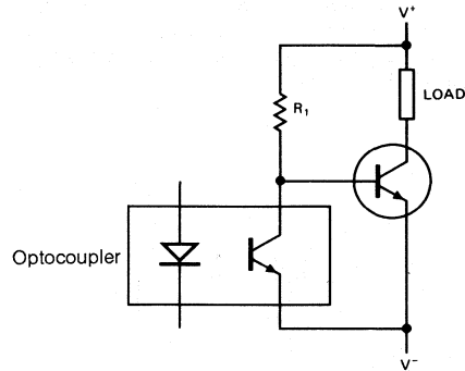
Figure 5A. NPN HV Booster
