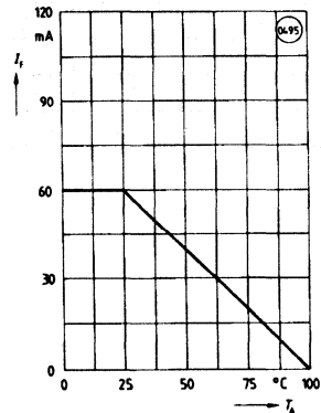
Figure 7. Permissible diode forward current versus ambient temperature
