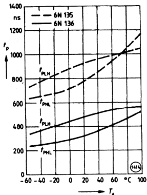
Delay times versus ambient temperature ( I_F=16\text{ mA} , V_{CC}=5\text{ V} , 6N135: R_L=4.1\text{ kW} , 6N136: R_L=1.9\text{ kW} )
