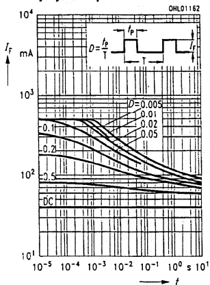
5D Permissible pulse handling capability I_F=f(t_p) , T_A=25^\circ\text{C} Duty cycle d -parameter
