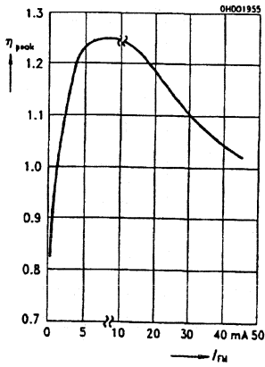
10E Relative efficiency I_V/I_{V(\dots mA)}=f(I_{FM}), T_A=25^\circ\text{C}
