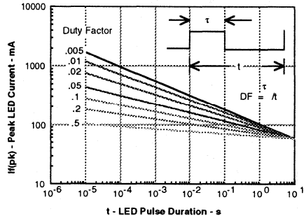
Figure 6. Peak LED current versus pulse duration, \tau
