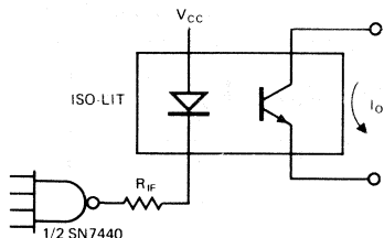
Figure 2. Buffer-Gate Drive
