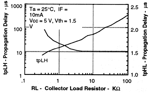
Figure 16. Propagation delay versus collector load resistor
