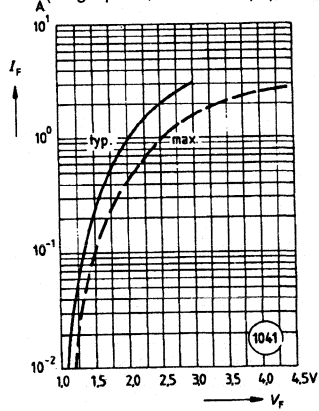
Forward current I_F=f(V_F) -SFH450V (Single pulse, duration=20μs) SFH450V
