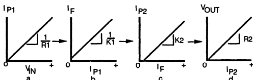
Figure 9. Positive Unipolar Photovoltaic Isolation Amplifier
