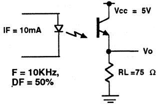
Figure 1. Non-saturated switching timing
