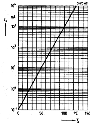
Dark current, I_R=f(T_A) , V_R=10V , E=0
