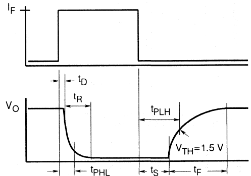
Figure 10. Switching Waveform
