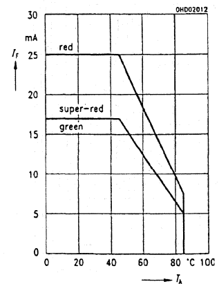
9A Maximum permissible forward current I_F=f(T_A)
