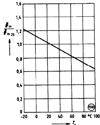
Temperature behavior—SFH752V
