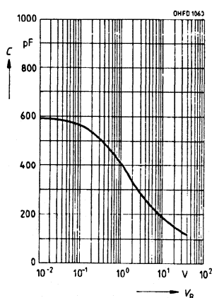
Capacitance C=f(V_R)
