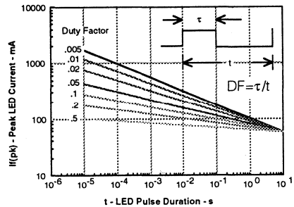
Figure 6. Peak LED current versus pulse duration, Tau
