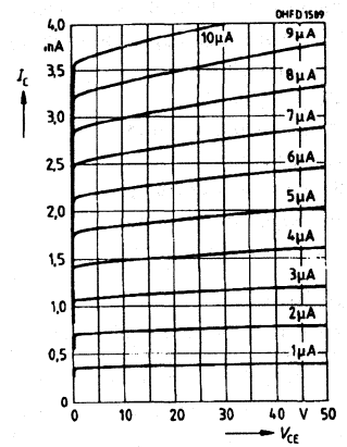
Output characteristics I_C=f(V_{CE}), I_B=\text{Parameter}
