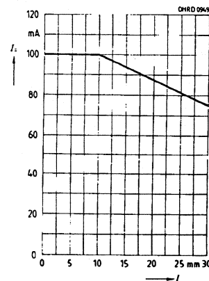
Forward current vs. lead length, package bottom and PC-board I_F = f(l) , T_A = 25^\circ\text{C}
