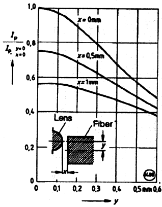
Coupling efficiency \Phi_{IN} versus alignment \Phi_{IN}/\Phi_{IN}(X, Y=0)=f(Y)
