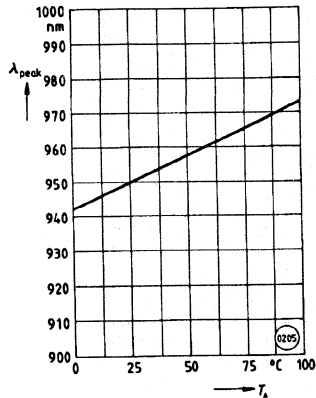
Peak wavelength-SFH450V
