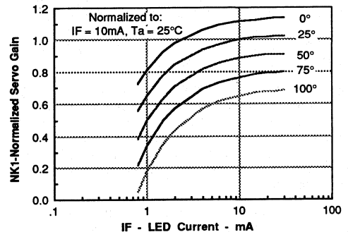
Figure 4. Normalized Servo Gain vs. LED Current
