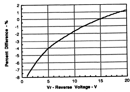
Figure 8a. Photoconductive Responsivity vs. Bias Voltage
