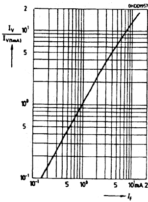
6B Relative luminous intensity I_v/I_{v(10\text{mA})}=f(I_f), T_A=25^\circ\text{C}
