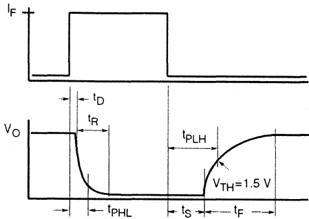
Figure 11. Switching timing
