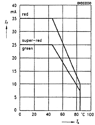
9C Maximum permissible forward current I_F=f(T_A)
