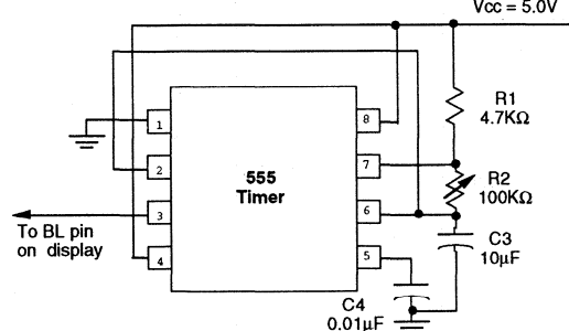
FIGURE 1a. FLASHING (Blanking) TIMING
