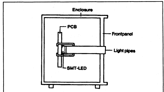
Figure 2. SMT TOPLED™ with light pipe to front panel
