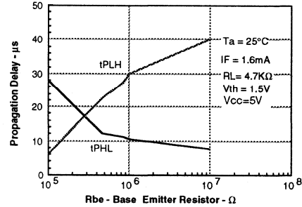
Figure 14. Propagation delay versus base emitter resistor
