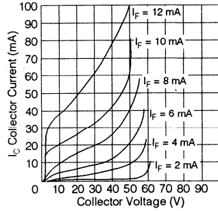
Figure 2. Transistor current versus voltage
