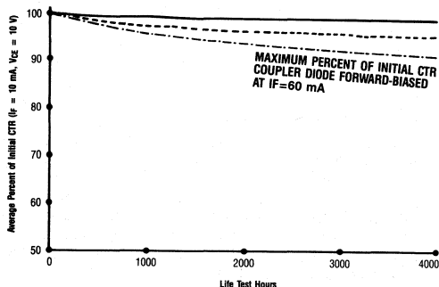
Figure 1. CTR Degradation vs. Time
