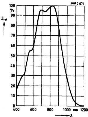
Relative spectral sensitivity S_{\text{rel}} = f(\lambda)
