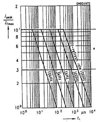
8K Permissible pulse handling capability I_F=f(t_p) , T_A=25^\circ\text{C} ; Duty cycle D =parameter
