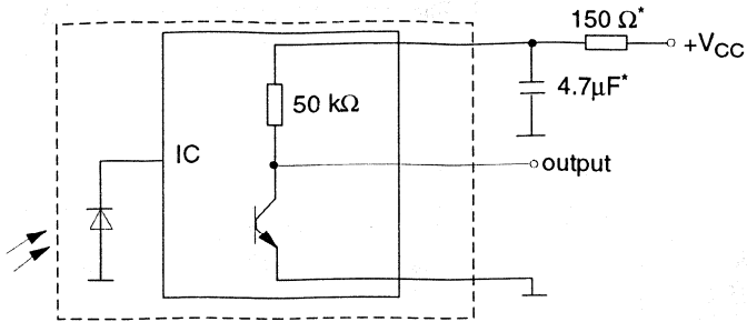
Figure 1. External Circuit
