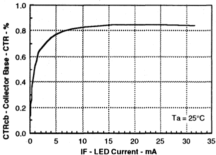
Figure 5. Collector base current transfer ratio versus LED current
