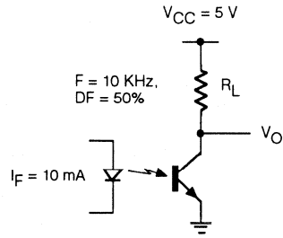
Figure 10. Switching schematic
