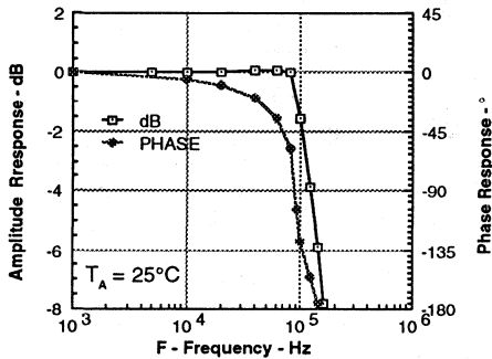
FIGURE 21. Amplitude and phase power supply control
