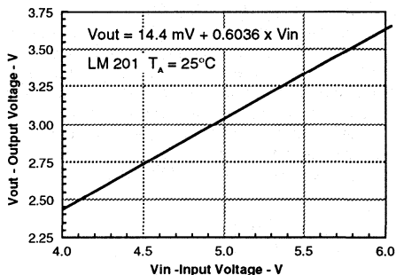
FIGURE 19. Transfer gain
