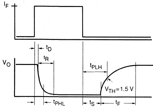
Figure 9. Switching Timing
