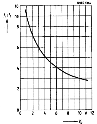
Switching times t_R / t_F = f(V_R) , R_L = 50 \Omega
