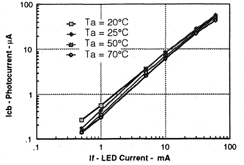
Figure 8. Photocurrent versus LED current
