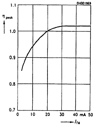
10G Relative efficiency I_V/I_{V(\dots mA)}=f(I_{FM}), T_A=25^\circ\text{C}
