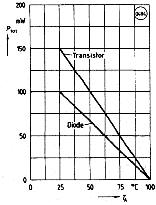
Figure 6. Permissible power dissipation for transistor and diode versus ambient temperature
