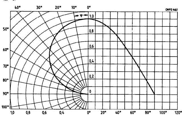
Directional characteristics S_{rel}=f(\psi)
