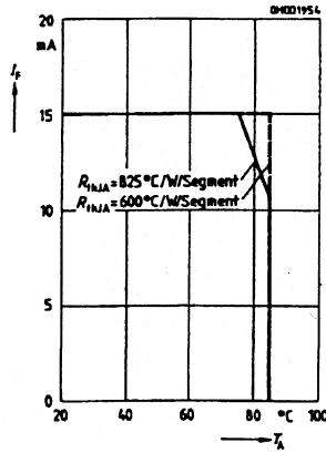
9H Maximum permissible forward current I_F=f(T_A)
