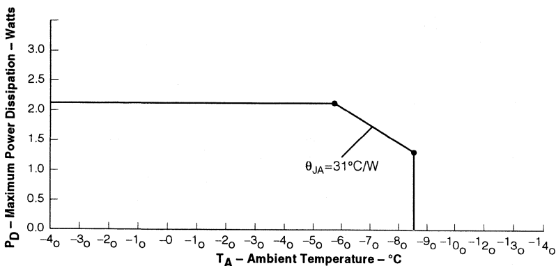
FIGURE 2. MAXIMUM POWER DISSIPATION VS. TEMPERATURE
