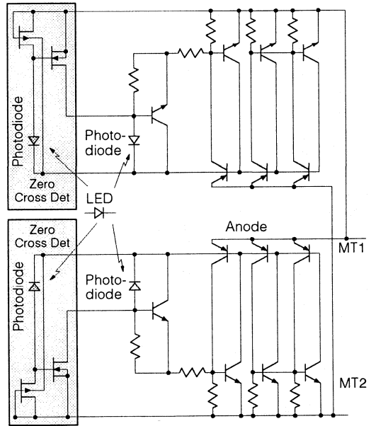
Figure 3. Schematic
