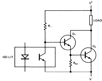
Figure 6A. NPN Darlington HV Booster
