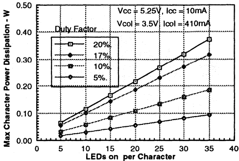
FIGURE 11. CHARACTER POWER DISSIPATION
