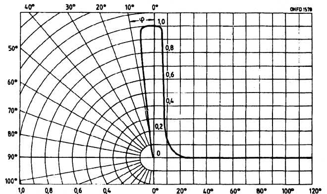
Directional characteristic S_{\text{rel}} = f(\phi)
