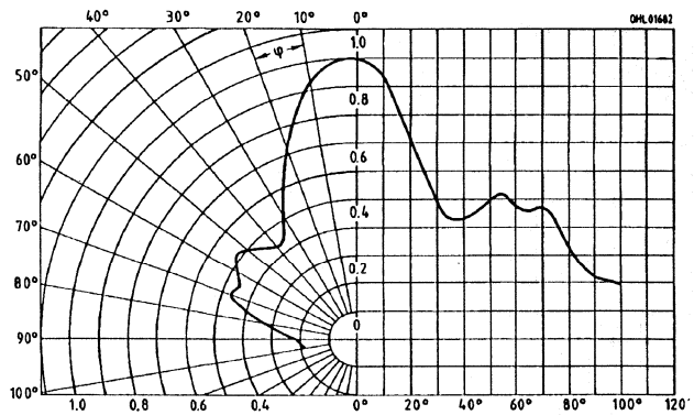
Radiation characteristics I_{rel}=f(\rho)
