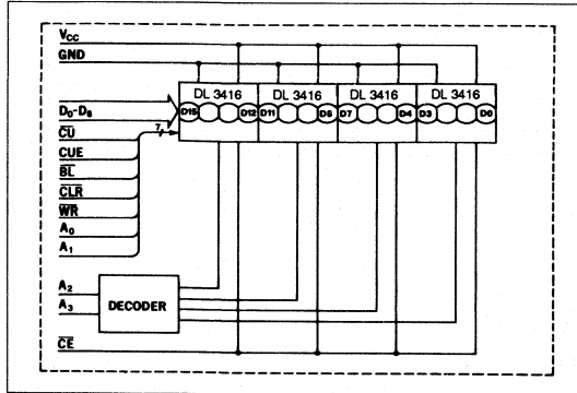
Figure 6. General Interface Circuit
