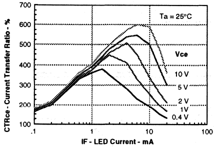
Figure 7. Current transfer ratio versus LED current
