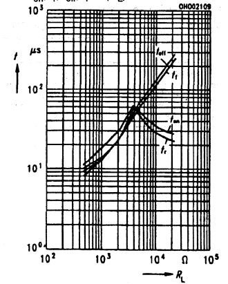
Figure 9. Switching times (typ.) T_A=25^\circ\text{C} , I_F=\pm 1\text{ mA} , V_{CC}=5\text{ V} t_{on}, t_r, t_{off}, t_f=f(R_L)
