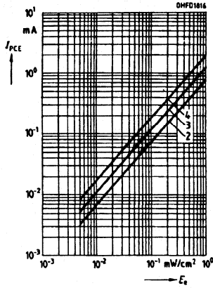
Photocurrent-BPX81 I_{PCE}=f(E_e)
