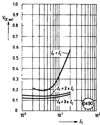
Saturation voltage versus collector current and modulation depth CNY17F-4 V_{CE sat} = f(I_C) ( T_A = 25^\circ\text{C} )
