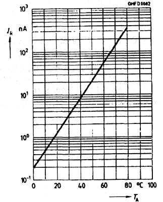
Dark current I_R=f(T_A) V_R=10 \text{ V}, E=0
