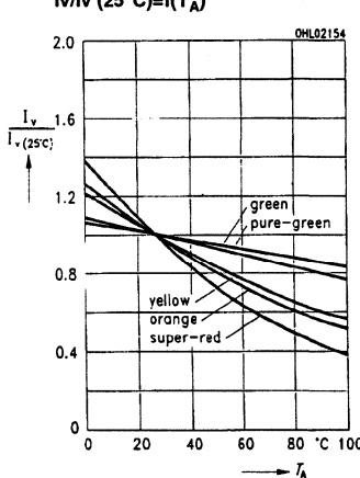
10E Rel. luminous intensity I_v/I_v(25^\circ\text{C})=f(T_A)
