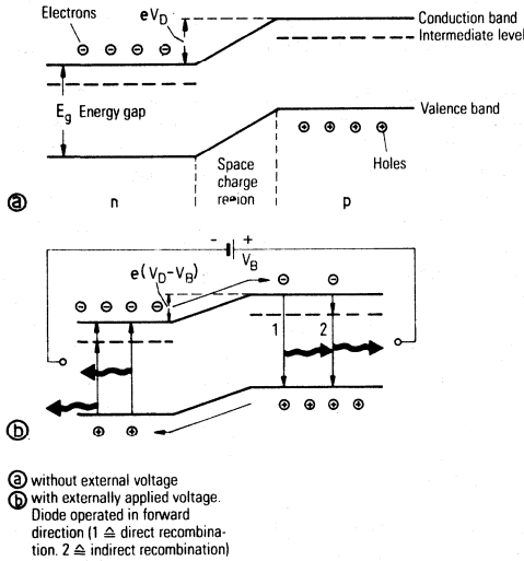
Fig. 2.1 The pn junction of a light emitting diode
