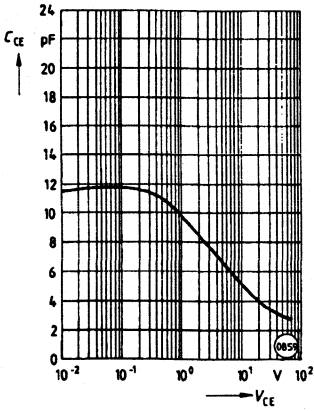
Figure 4. Transistor capacitance (typ.) Capacitance versus collector-emitter voltage ( T_A=25^\circ\text{C} , f=1\text{ MHz} )
