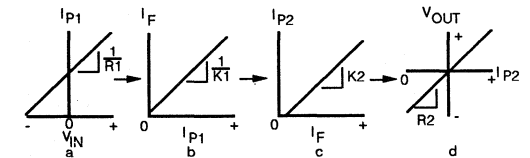
Figure 19. Prebiased Photovoltaic Isolation Amplifier Transfer Characteristics
