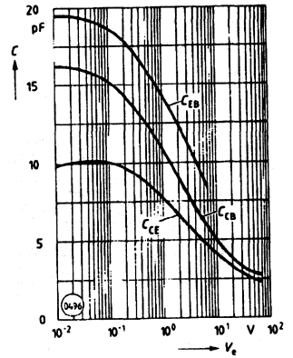
Figure 18. Transistor capacitance C=f(V_{CE}) ( T_A=25^\circ\text{C} , f=1\text{ MHz} )
