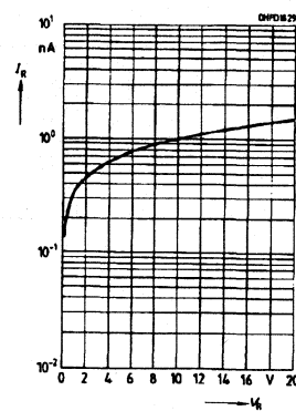
Dark current I_R=f(V_R), E=0
