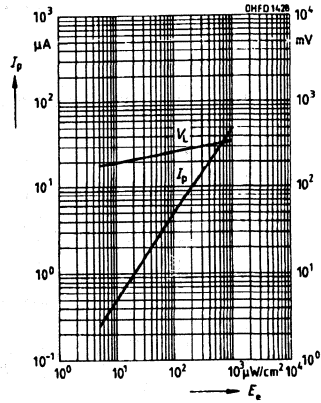
Photocurrent I_P=f(E_E, V_{REL}=5 V(\lambda)) Open circuit voltage V_O=f(E_E)
