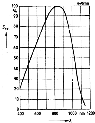
Relative spectral sensitivity—SFH229P S_{REL}=f(\lambda)
