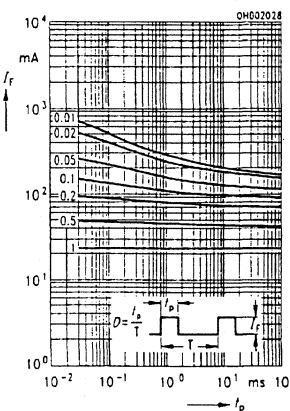
8F Permissible pulse handling capability I_F=f(t_p) , T_A=25^\circ\text{C} ; Duty cycle D=\text{parameter}
