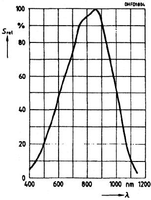
Relative spectral sensitivity—SFH317 S_{REL}=f(\lambda)
