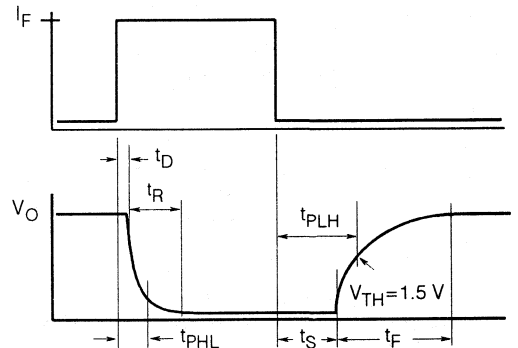
Figure 14. Switching waveform
