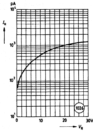
Dark current I_R=f(V_R), T_A=25^\circ\text{C}
