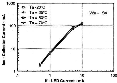
Figure 5. Collector current versus LED current
