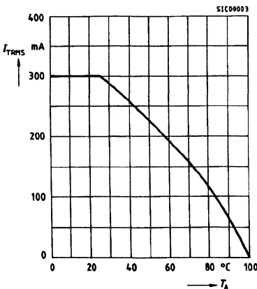
Figure 8. Current reduction
