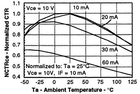
Figure 7. Normalized saturated current transfer ratio versus temperature and LED current
