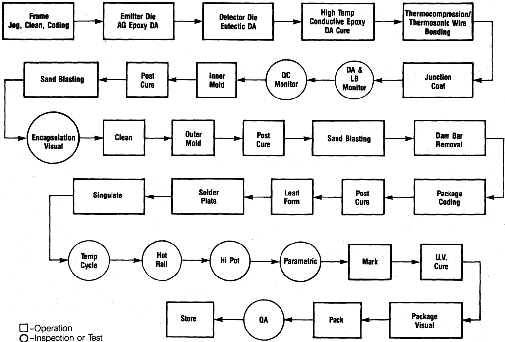
Figure 4. Coupler Process Flow & Inspections
