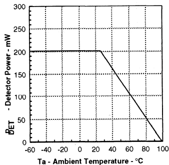
Figure 6. Detector power versus ambient temperature
