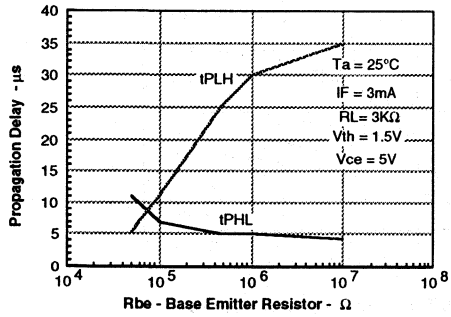
Figure 15. Propagation delay versus base emitter resistor
