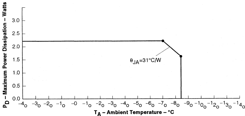
FIGURE 2. MAXIMUM POWER DISSIPATION VERSUS TEMPERATURE
