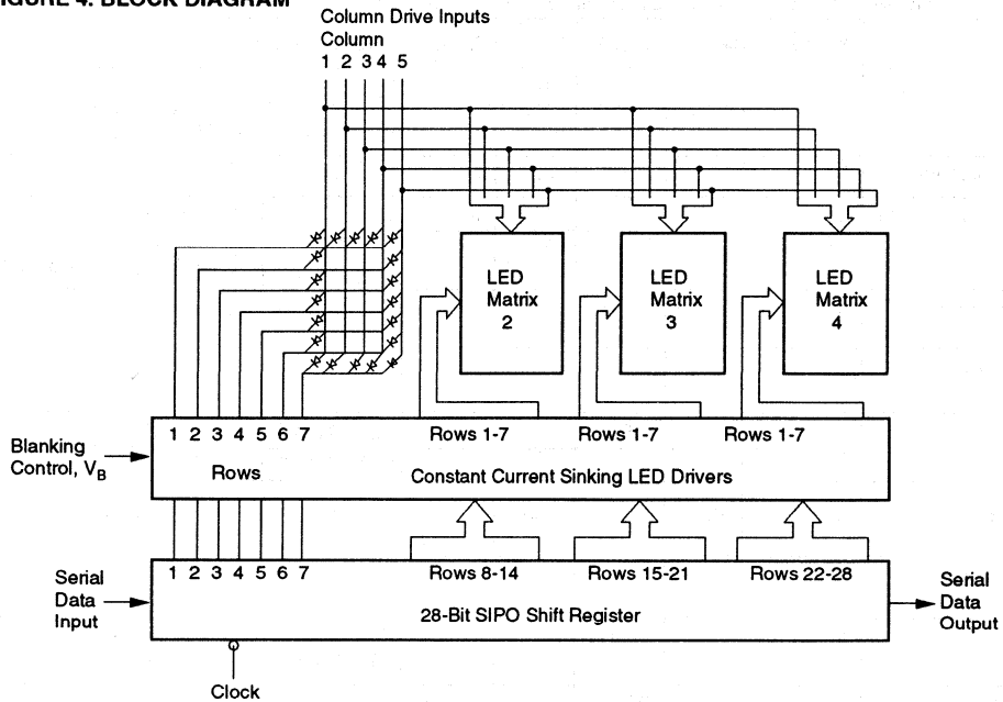
FIGURE 4. BLOCK DIAGRAM
