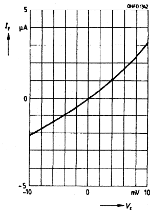
Zero crossover I_F=f(V_R) , E=0
