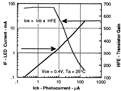
Figure 12. Transfer curve
