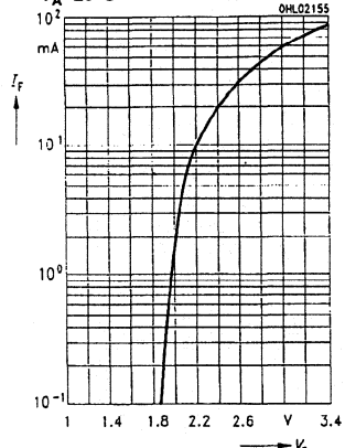
3C Forward current I_F=f(V_F) T_A=25^\circ\text{C}
