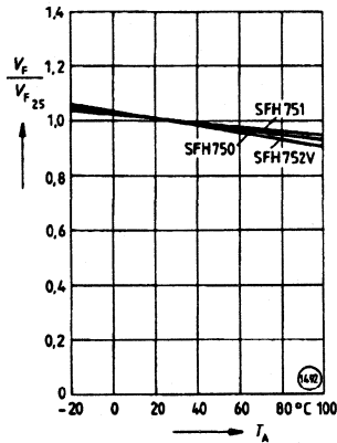
Temperature behavior—SFH752V
