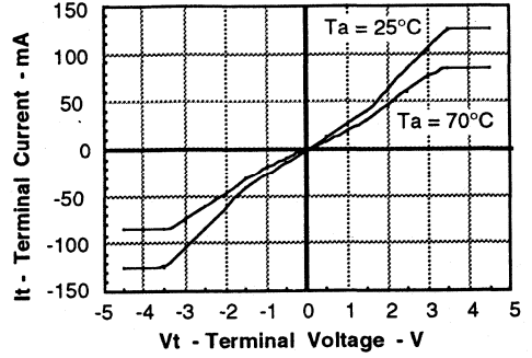
Figure 2. Terminal current versus terminal voltage
