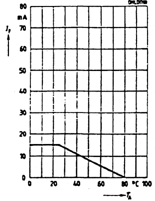
6H Max. Permissible forward current I_F=f(T_A)
