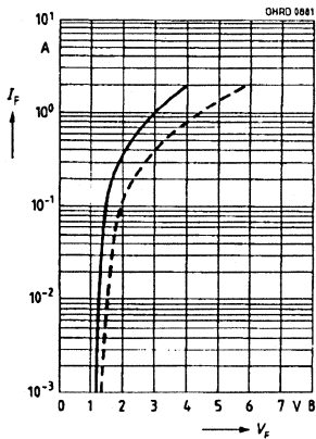
Forward current I_F = f(V_F) Single pulse, \tau = 20 \mu
