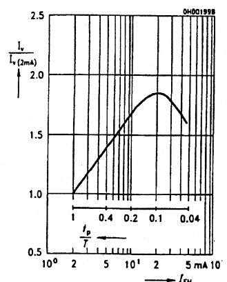
10A Relative efficiency I_V/I_V(\dots mA)=f(I_{FM}) , T_A=25^\circ\text{C}
