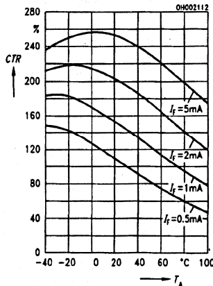
Figure 2. Current transfer ratio (typ.) V_{CE}=1.5\text{ V} , CTR=f(T_A)
