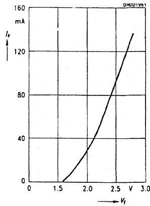
3B Forward current I_F=f(V_F) , T_A=25^\circ\text{C}
