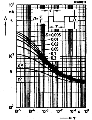
Permissible pulse handling capability I_F = f(\tau) , T_C = 25^\circ C duty cycle D = \text{Parameter}
