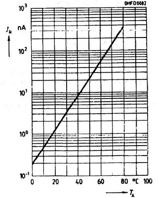
Dark current I_R = f(T_A)
