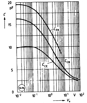
Transistor capacitance C=f(V_e) ( T_A=25^\circ\text{C} , f=1 \text{ MHz} )
