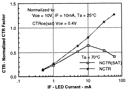
Figure 3. Collector current versus diode forward current
