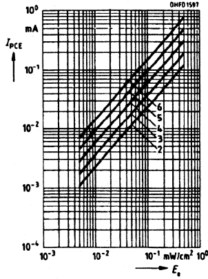
Photocurrent I_{PCE}=f(E_e), V_{CE}=5 V
