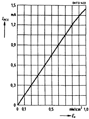
Forward current I_{PCE}=f(E_e), V_{CE}=5\text{ V}
