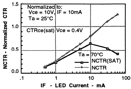
Figure 10. Collector-emitter current versus temperature and LED current
