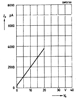
Dark current I_R=f(V_R) T_A=25^\circ\text{C}, E=0
