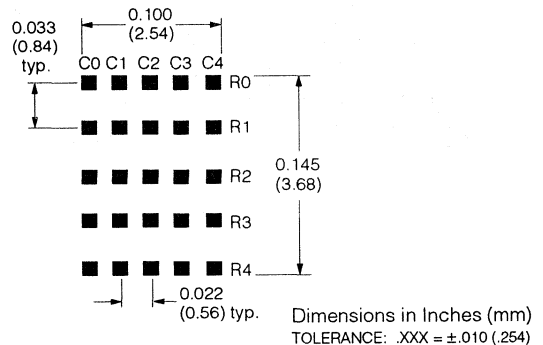
FIGURE 5. DOT MATRIX FORMAT
