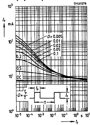
5F Permissible pulse handling capability I_F=f(t_p) , T_A=25^\circ\text{C} Duty cycle d -parameter
