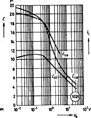
Capacitance C = f(V_R), f = 1 \text{ MHz}, E_V = 0
