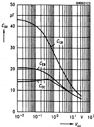
Figure 10. Transistor capacitance (typ.) T_A=25^\circ\text{C} , f=1\text{ MHz} , C_{CE}=f(V_{CE}) C_{CB}=f(V_{CB}) , C_{CEB}=f(V_{EB})
