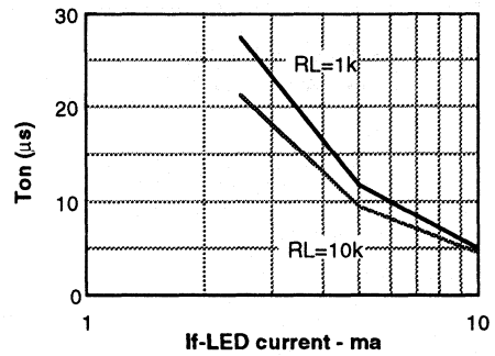
Figure 11. Tplh versus forward current
