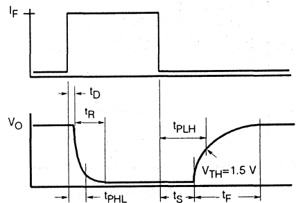
Figure 14. Switching timing
