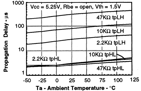
Figure 23. Propagation delay versus temperature and collector load resistance for I_F=5\text{ mA}
