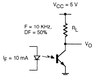
Figure 15. Switching schematic
