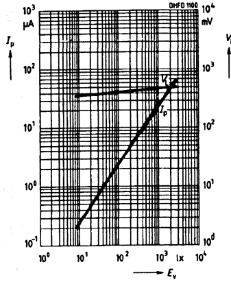
Photocurrent I_P=f(E_V) V_R=5 V Open circuit voltage V_G=f(E_V)
