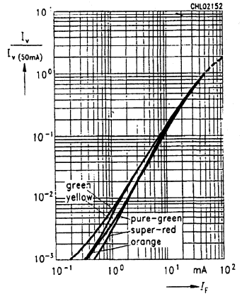
4F Rel. luminous intensity I_V/I_V(50\text{ mA}) = f(I_F)
