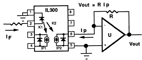
Figure 5a. Photovoltaic Amplifier Configuration
