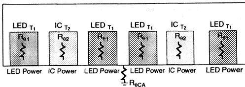
FIGURE 5. THEMAL MODEL
