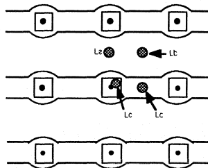
Figure 3. Points for Luminous Sterance Measurement
