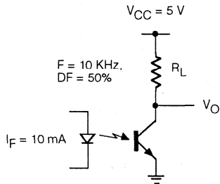
Figure 15. Switching schematic
