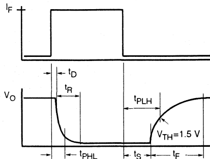
Figure 9. Switching waveform
