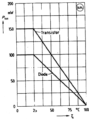
Permissible power dissipation transistor and diode P_{tot}=f(T_A)
