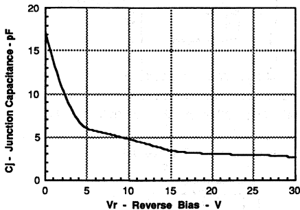
Figure 10a. Photodiode Junction Capacitance vs. Reverse Voltage
