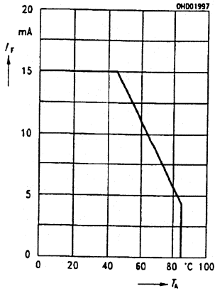
9G Maximum permissible forward current I_F=f(T_A)
