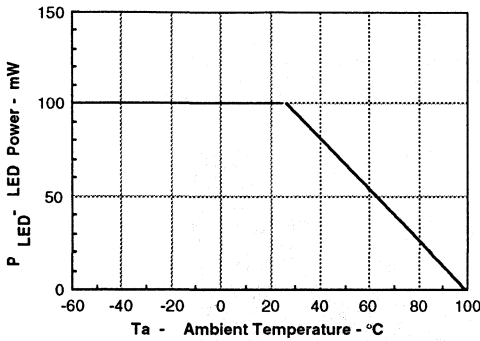
Figure 6. Maximum LED power dissipation
