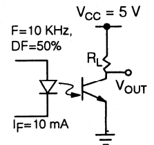
Figure 10. Switching schematic
