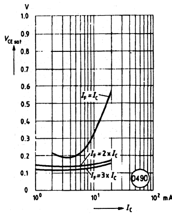
Figure 14. Saturation voltage versus collector current and modulation depth SFH600-3 V_{CEsat}=f(I_C) ( T_A=25^\circ\text{C} )
