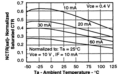
Figure 7. Normalized saturated current transfer ratio versus temperature and LED current
