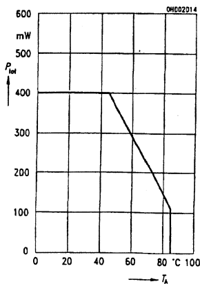
11A Total power dissipation P_{TOT}=f(T_A)
