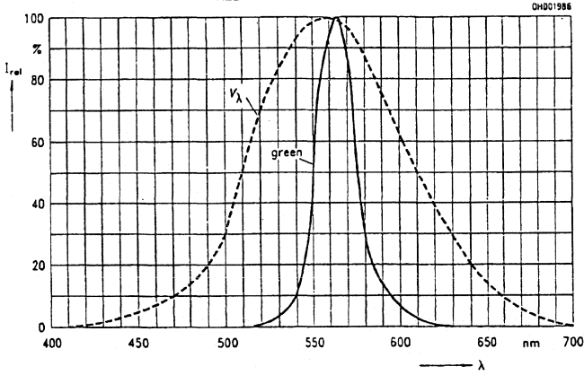
1E Relative spectral emission I_{REL}=f(\lambda) ; T_A=25^\circ\text{C} , V(\lambda) =standard eye response curve
