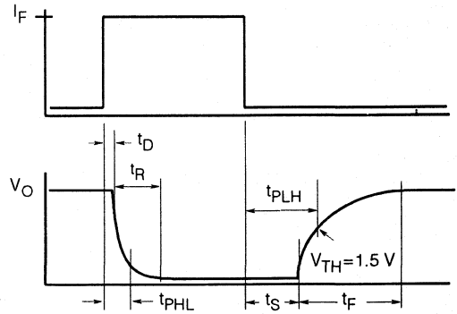
Figure 6. Switching timing
