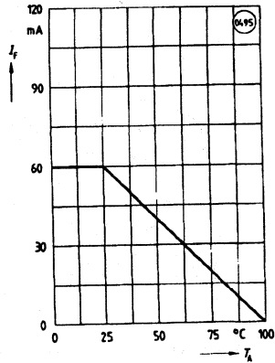
Figure 17. Permissible forward current diode I_F=f(T_A)
