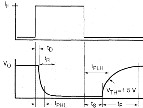
Figure 8. Switching waveforms
