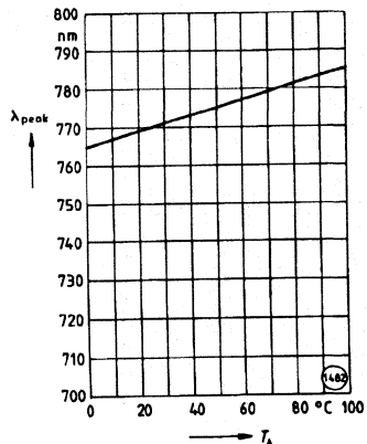
Peak wavelength-SFH452V
