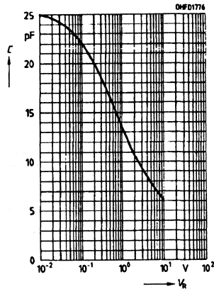
Capacitance C=f(V_R)
