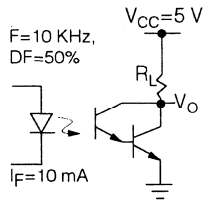
Figure 7. Switching schematic
