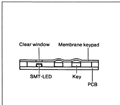
Figure 8. LED behind membrane keypad.
