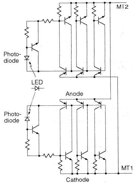
Figure 11. Schematic
