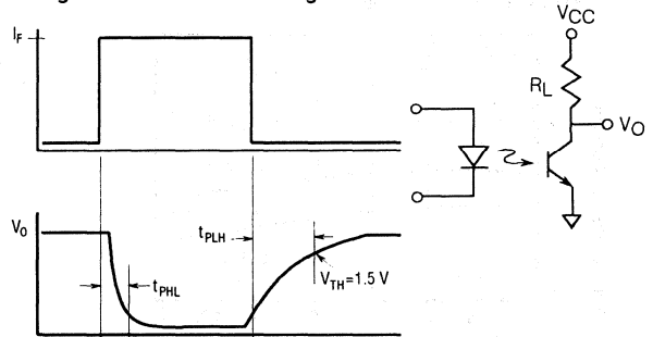
Figure 16. Saturated Switching
