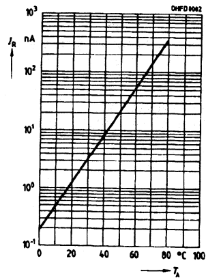
Dark current, I_R=f(T_A) , V_R=1 V, E=0
