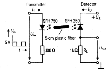
Fig. 6 Basic circuit to operate light-link optocouplers
