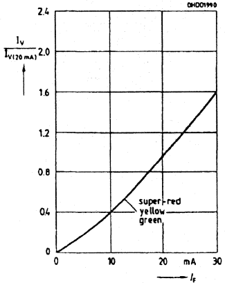
6G Relative luminous intensity I_v/I_{v(10\text{mA})}=f(I_f), T_A=25^\circ\text{C}
