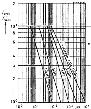
8L Permissible pulse handling capability I_F=f(t_p) , T_A=25^\circ\text{C} ; Duty cycle D =parameter
