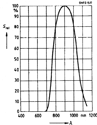
Relative spectral sensitivity—SFH229PF S_{REL}=f(\lambda)
