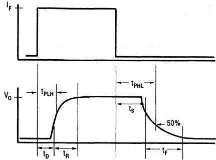
Figure 3. Non-saturated switching timing
