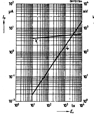
Photocurrent I_p = f(E_s) , V_R = 5\text{ V} Open-circuit voltage V_L = f(E_s)
