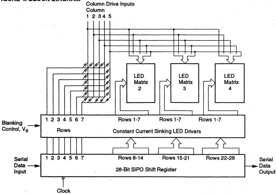
FIGURE 4. BLOCK DIAGRAM
