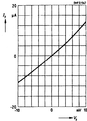
Zero crossover I_F=f(V_F) , E=0
