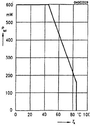
11C Total power dissipation P_{TOT}=f(T_A)
