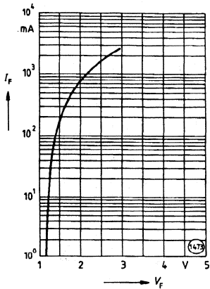
Forward voltage-SFH452V
