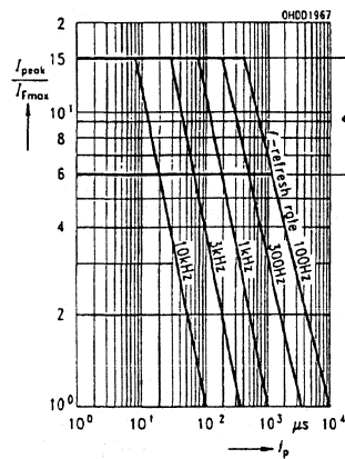
8I Permissible pulse handling capability I_F=f(t_p) , T_A=25^\circ\text{C} ; Duty cycle D =parameter
