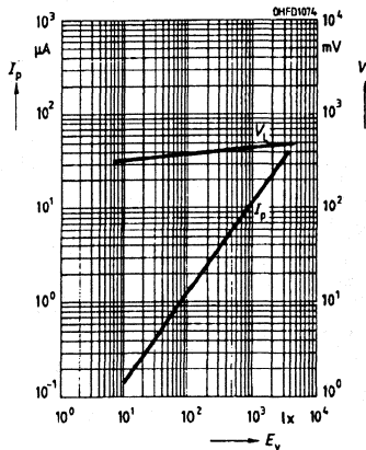
Photocurrent I_P=f(E_V) , V_R=5 V Open circuit voltage V_0=f(E_V)
