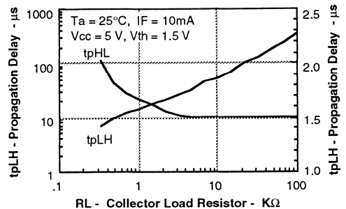
Figure 8. Propagation delay versus collector load resistor
