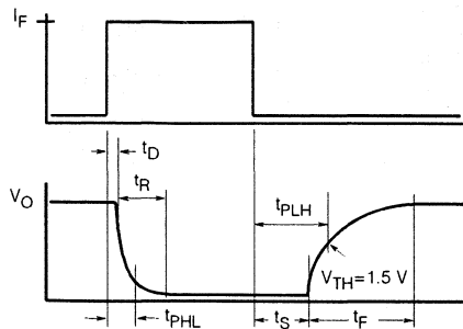
Figure 14. Switching waveform
