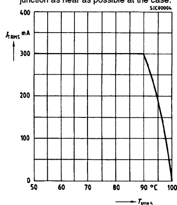
Figure 9. Current reduction
