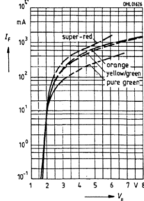
3F Forward current I_F=f(V_F) T_A=25^\circ\text{C}
