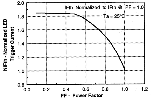
Figure 2. Normalized LED trigger current versus power factor
