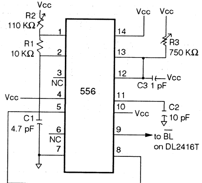
FIGURE 2. DIMMING CIRCUIT FOR DL2416T USING A 556
