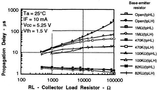
Figure 29. Propagation delay versus collector load and base-emitter resistance for I_f=10 mA
