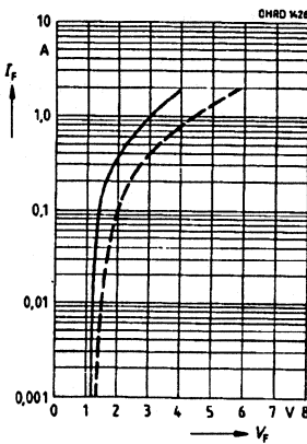
Forward current—IRL 81A I_F=f(V_F)
