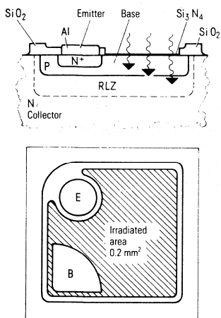
Fig. 1.4 Bipolar phototransistor
