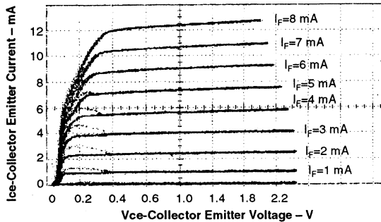
Figure 7. Collector emitter current versus collector emitter voltage
