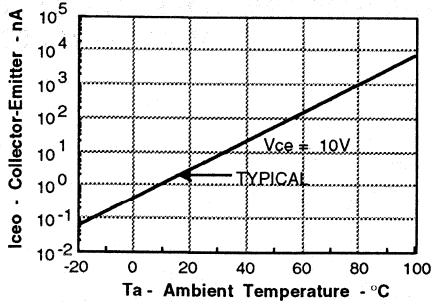
Figure 15. Collector-emitter leakage versus temperature
