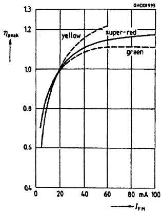
10H Relative efficiency I_V/I_{V(\dots mA)}=f(I_{FM}), T_A=25^\circ\text{C}
