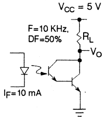
Figure 9. Switching schematic
