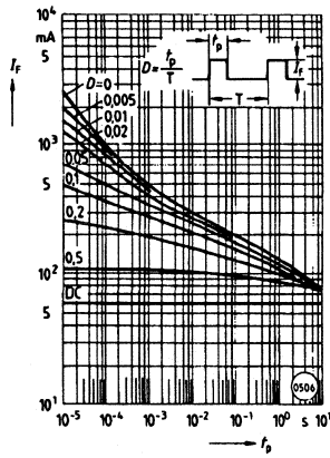
Figure 5. Permissible pulse handling capability. Forward current versus pulse width (Pulse duty factor D=\text{parameter} , T_A=25^\circ\text{C} )
