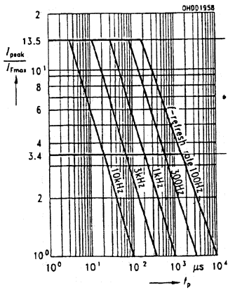
8H Permissible pulse handling capability I_F=f(t_p) , T_A=25^\circ\text{C} ; Duty cycle D =parameter
