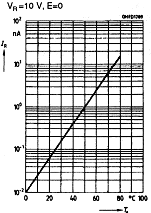
Dark current I_R = f(T_A)
