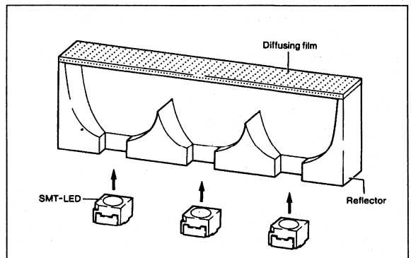
Figure 10. SMT-TOPLED™ illuminating a large area.
