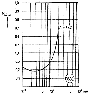
Figure 11. Saturation voltage versus collector current and modulation depth SFH600-0 V_{CEsat}=f(I_C) ( T_A=25^\circ\text{C} )
