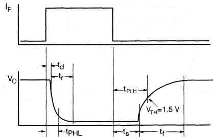
Figure 14. Switching Waveform
