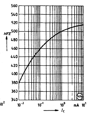
Current gain HFE = f(I_C), V_{CE} = 5 \text{ V}, T_A = 25^\circ \text{C}
