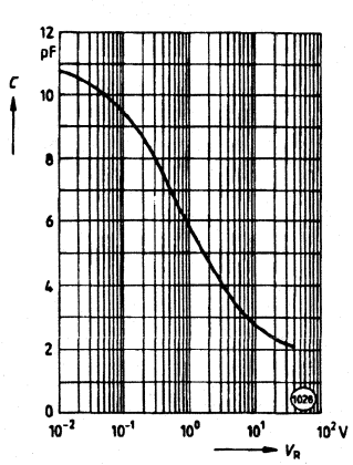
Capacitance C=f(V_R), f=1\text{ MHz}, E_V=0
