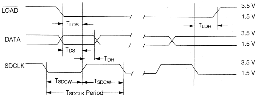
FIGURE 1. DATA WRITE CYCLE
