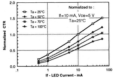
Figure 6. Normalized CTRcb
