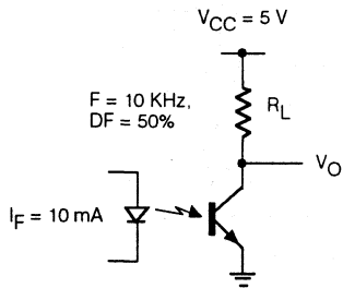
Figure 17. Switching schematic
