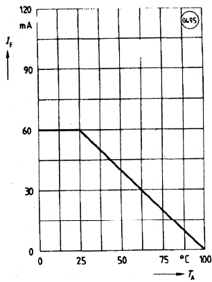
Permissible forward current diode I_F = f(T_A)
