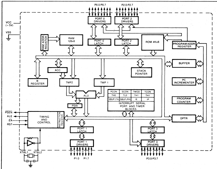
FIGURE 1 — 8031 BLOCK DIAGRAM
