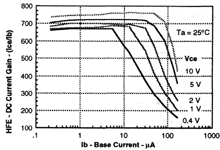
Figure 10. Transistor current gain versus base current
