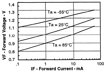
Figure 5. Forward voltage versus forward current
