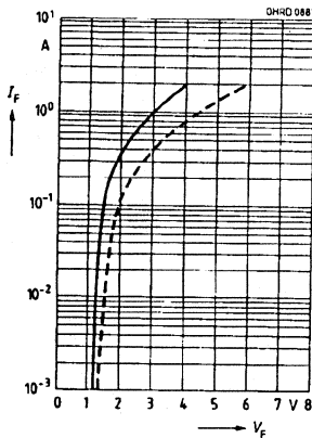
Forward current I_F = f(V_F) Single pulse, \tau = 20 \mu\text{s}
