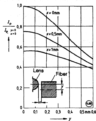
Coupling efficiency I_{P(in)} \text{ versus alignment } I_{C(x, y=0)} = f(y)
