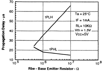
Figure 13. Propagation delay versus base emitter resistor
