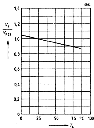
Forward voltage V_F/V_{F25} = f(T_A)
